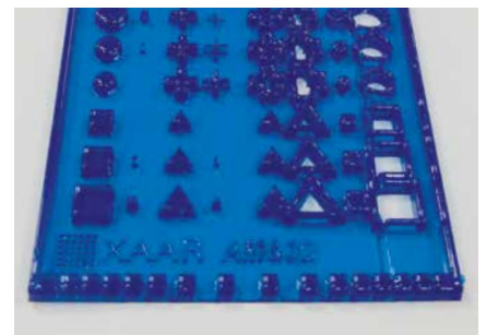
2.5D resolution test sample made with photopolymer (40 mPa.s @ 50C) printed using Xaar 1003 GS12 printhead with standard three-cycle jetting
