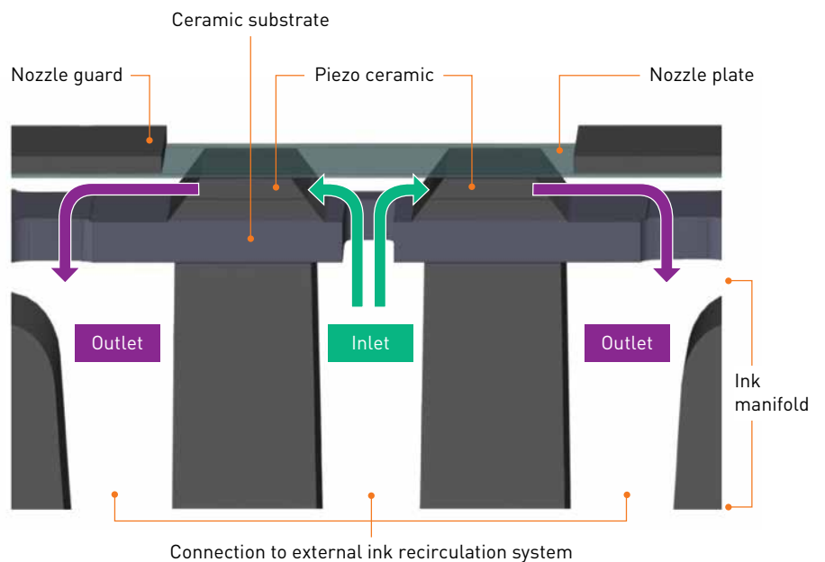
Figure 2a: Schematic of Xaar TF Technology showing the path of fluid into the piezoceramic channels, directly behind the nozzles, and out again
