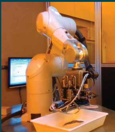
A Xaar jetting test rig with a Staubli robot arm (at the Iprint Institute for Printing, Switzerland) is shown on the left with the close-up on the right showing a Xaar 1003 printhead mounted on the robot arm for jetting at high levels of acceleration and deceleration 11
