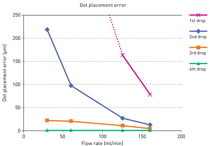
Figure 7: Dot placement errors for the first 4 dots from the burst of 10 drops as a function of the flow rate (30, 60, 125 and 160 ml/min). Idling time before the burst of 10 drops was 5 minutes in all cases.
