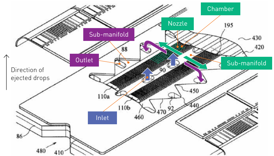
Figure 2: Xaar original patent on ink recirculating printhead with open architecture for strong recirculating ink flow
