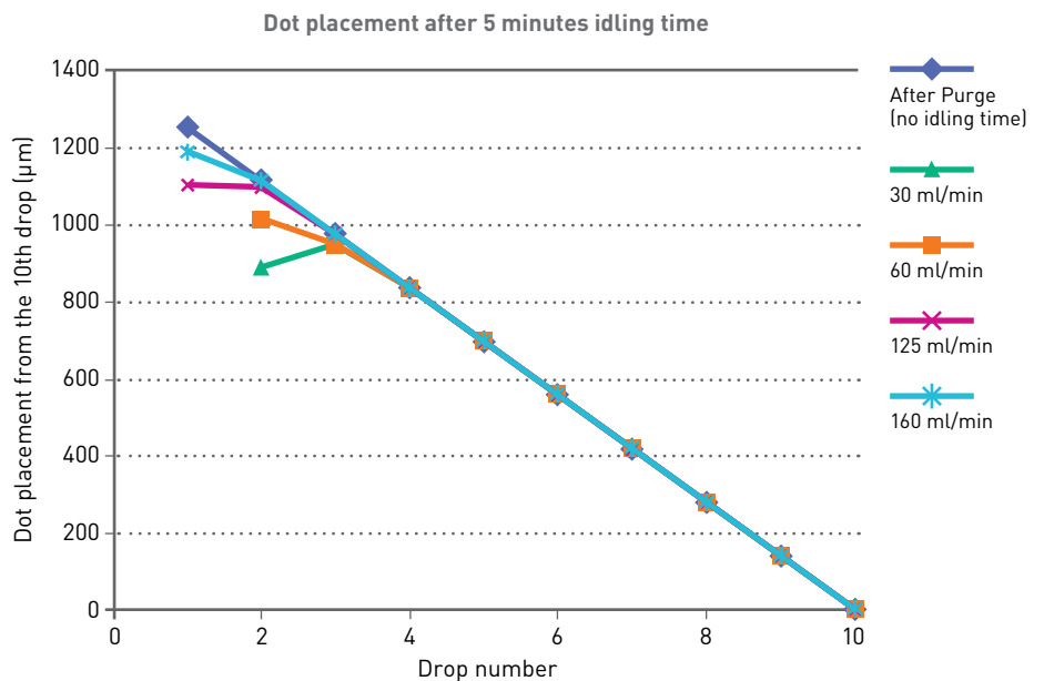
Figure 6: Dot placement after 5 minutes idling time where the position of each dot relative to the position of the dot from the 10th drop in a burst of 10 drops is measured. The test pattern used had a clear pixel between each dot in a burst and 200 clear pixels between bursts
