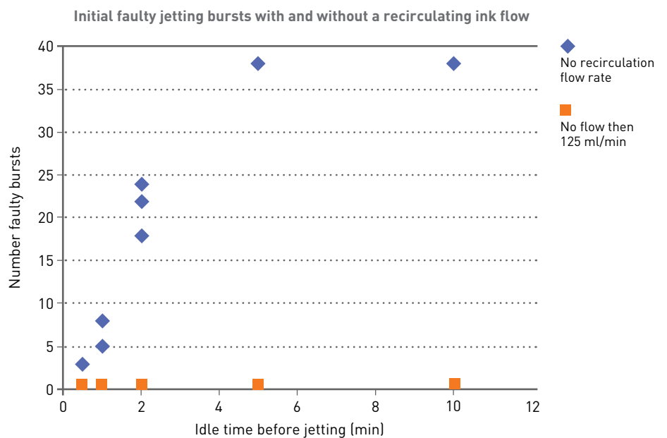
Figure 9: Initial jetting bursts at zero flow vs nominal. The blue diamonds represent the number of faulty 10-drop bursts before full recovery (i.e. the first burst with no defects)
