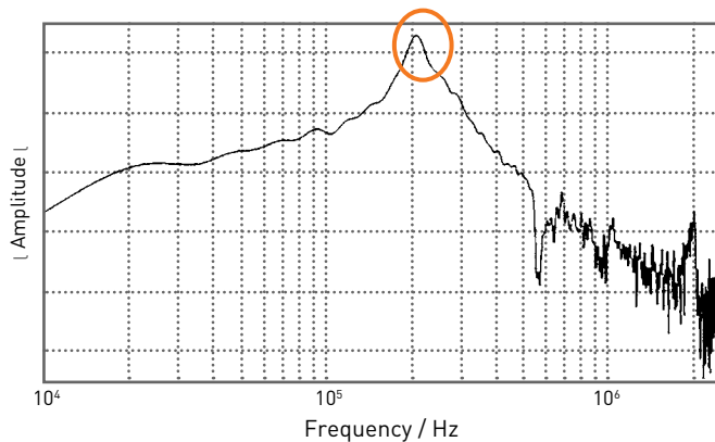
Figure 5: The plot of acoustic signal amplitude as a function of acoustic resonator frequency (above) shows a single peak for a bubble-free actuator channel. Equivalent plots (right) show the impact on the actuator acoustics for different bubble positions in the actuator channel ( a = channel centre; b = 0.2 mm from centre; c = 0.6 mm from centre)
